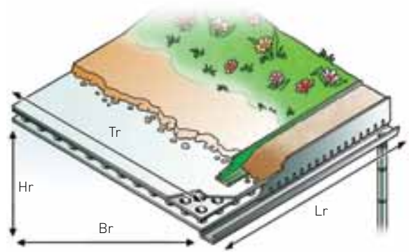
Figure 1. Roof dimensions
